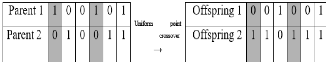
Figure 2. Example of Uniform Crossover
