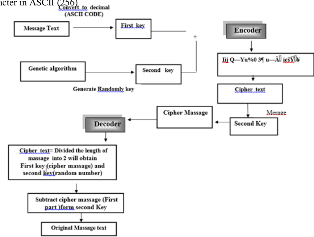
Figure ( 1 ):generic process of encoding and decoding.
